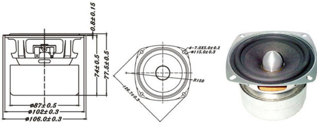
4" PAPER CONE/FULL RANGE, WOOFER
